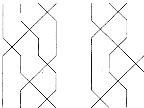
Fig. 1. Two expressions for W_4(z, \lambda) .
